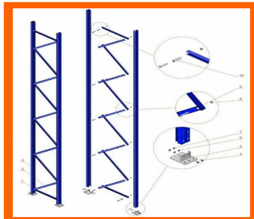
Racks Frames
