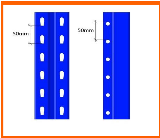
Racks Uprights
